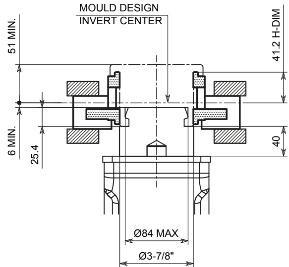
MINIMUM LIMIT FOR INCREASED BOTTOM PLATE
