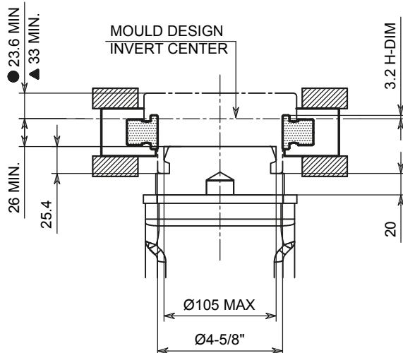
MINIMUM LIMIT FOR STANDARD BOTTOM PLATE
