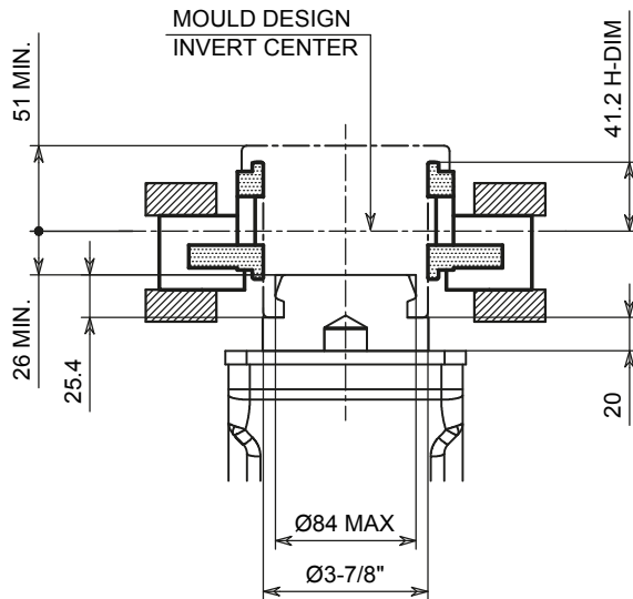
MINIMUM LIMIT FOR STANDARD BOTTOM PLATE
