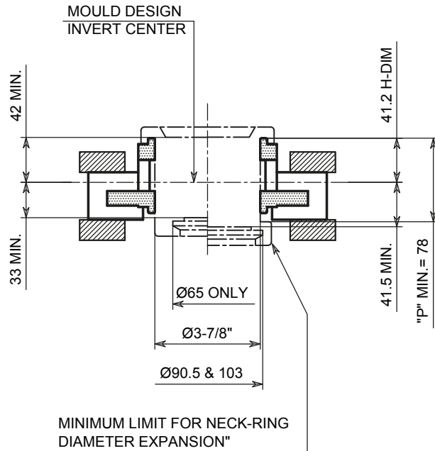
1-1/2" OFFSET MOULD HOLDER
