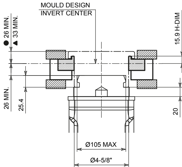
MINIMUM LIMIT FOR STANDARD BOTTOM PLATE
