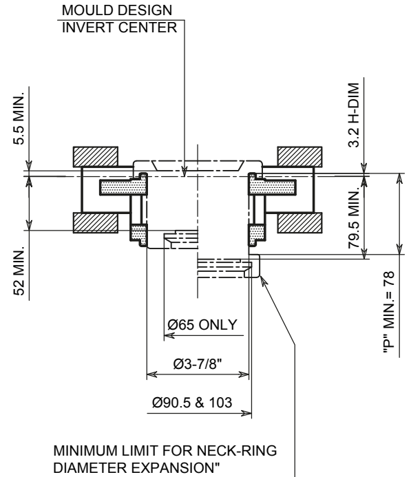
1-1/2" OFFSET MOULD HOLDER
