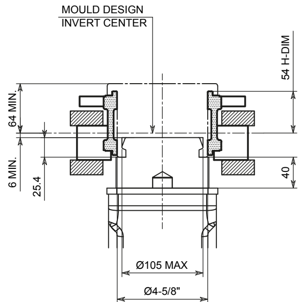
MINIMUM LIMIT FOR INCREASED BOTTOM PLATE
