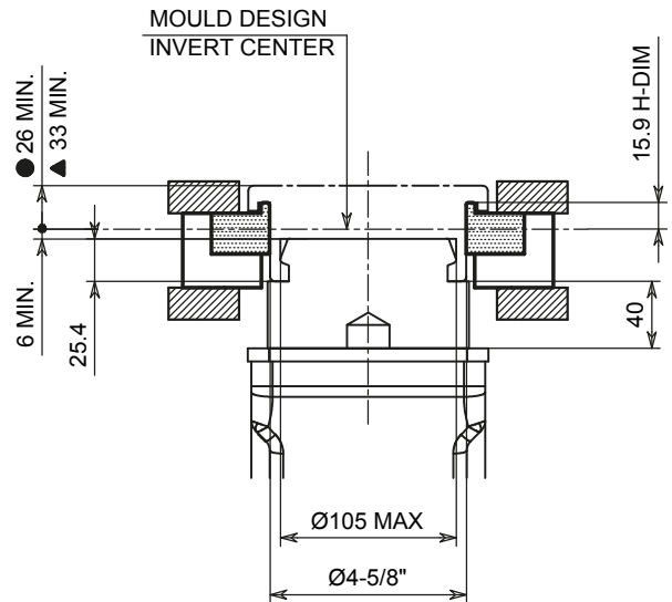
MINIMUM LIMIT FOR INCREASED BOTTOM PLATE
