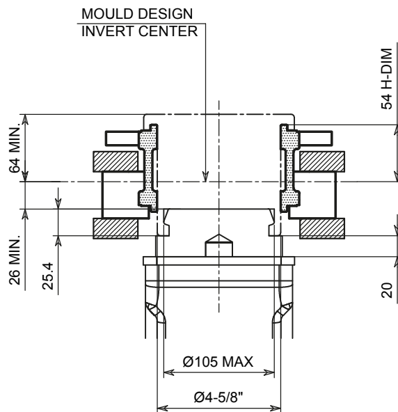
MINIMUM LIMIT FOR STANDARD BOTTOM PLATE
