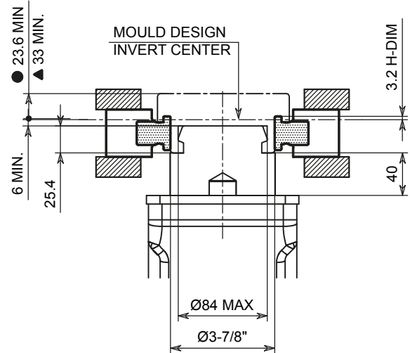
MINIMUM LIMIT FOR INCREASED BOTTOM PLATE
